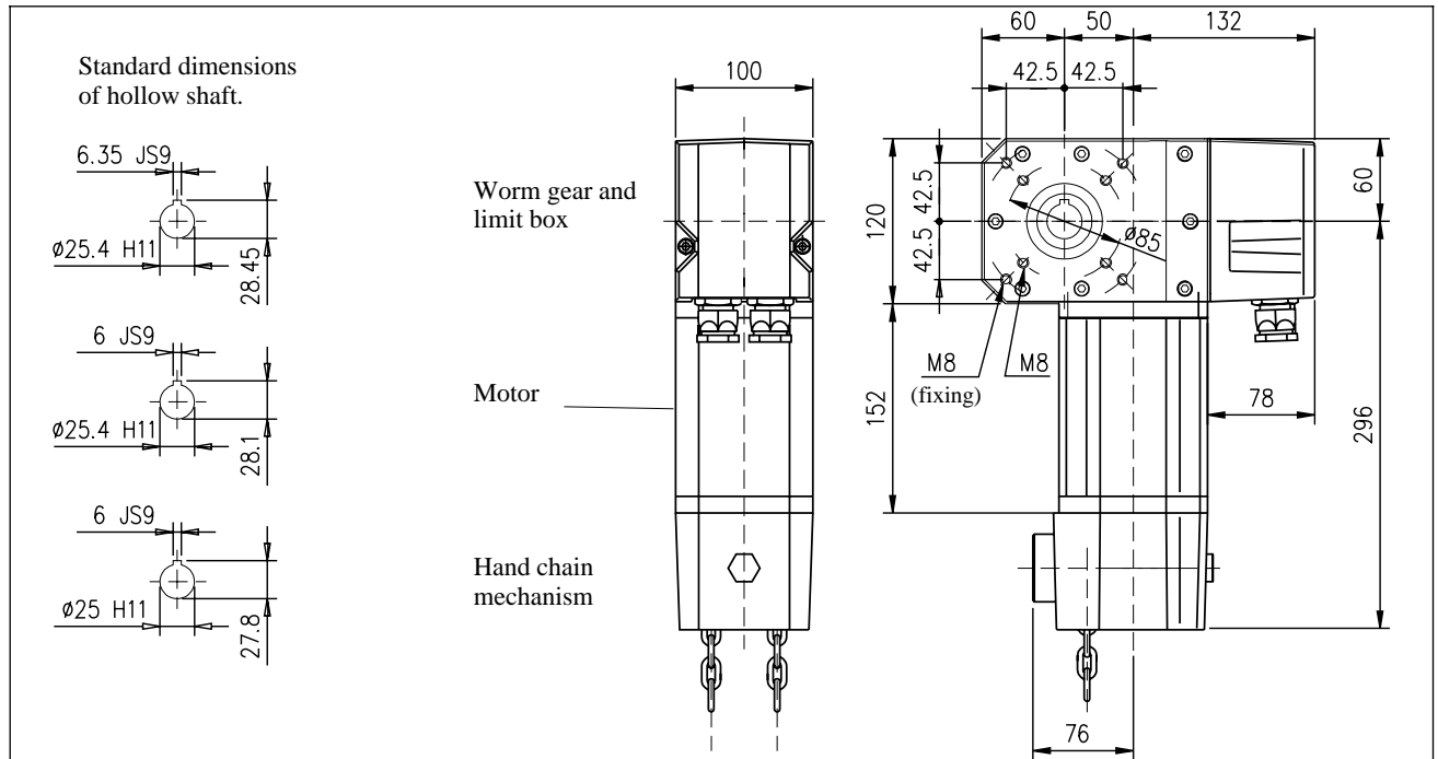
Fig. 1. Hollow shaft operator KVR5 with hand chain device.
