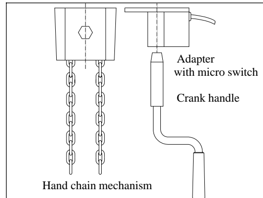
Fig. 3. Manual operation.
