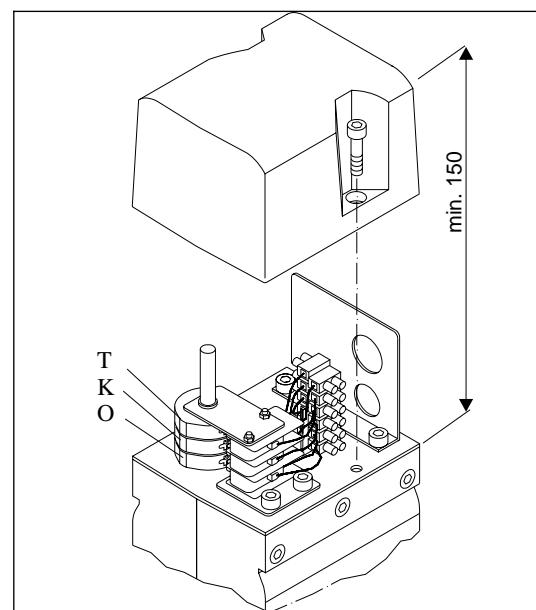
Fig. 4. Limit switches.
